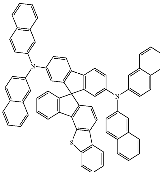
[Chemical Formula B-23]
