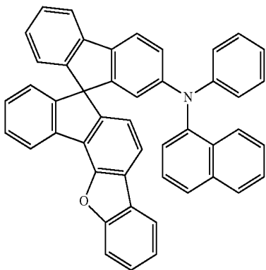
[Chemical Formula A-1]
