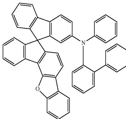
[Chemical Formula A-13]
