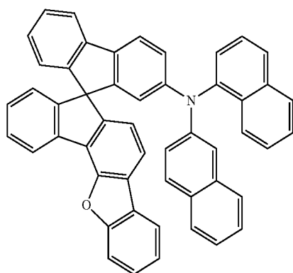
[Chemical Formula A-40]
