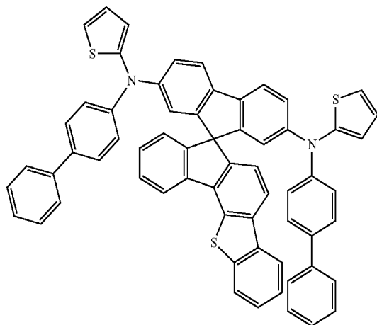
[Chemical Formula B-38]
