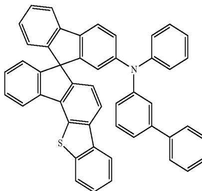
[Chemical Formula A-42]
