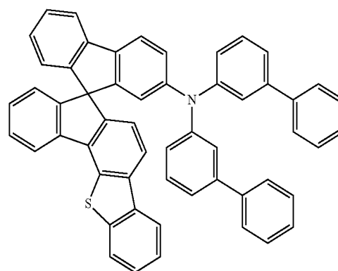
[Chemical Formula A-44]
