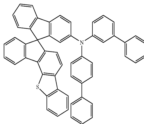
[Chemical Formula A-43]
