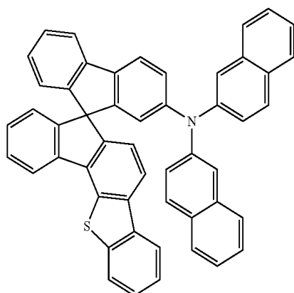
[Chemical Formula A-39]
