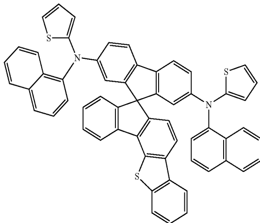
[Chemical Formula B-40]
