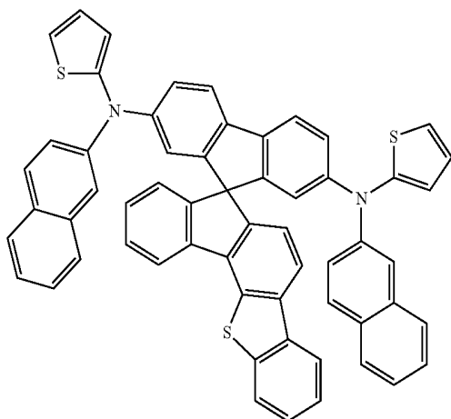
[Chemical Formula B-39]
