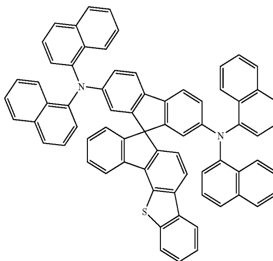
[Chemical Formula B-23]
