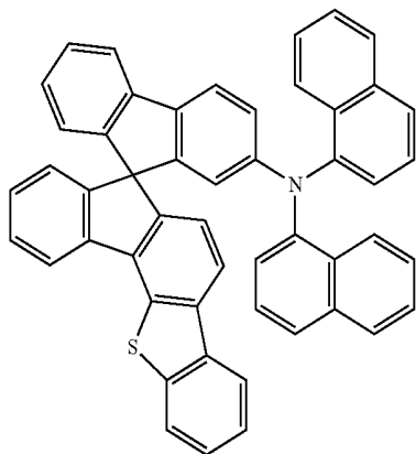
[Chemical Formula A-38]
