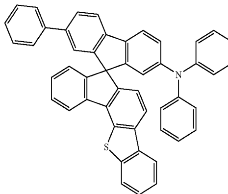
[Chemical Formula A-69]
