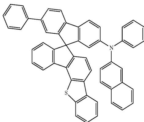
[Chemical Formula A-72]
