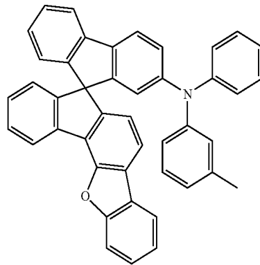
[Chemical Formula A-13]
